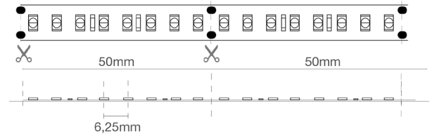
8 LED (14,4W)
